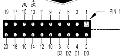
SNAP DIGITAL MODULE BASE CONTROL CONNECTOR (BOTTOM VIEW)
